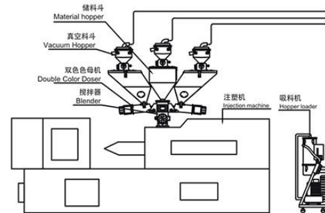
INSTALLATION DIAGRAM
