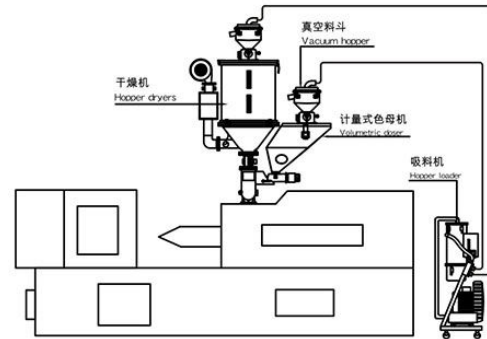
INSTALLATION DIAGRAM
